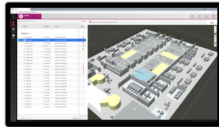
insoft Assets
