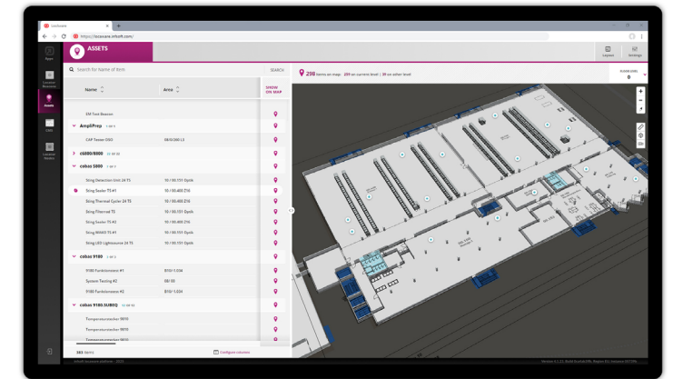
insoft Assets
