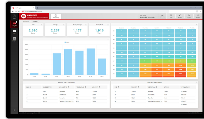
insoft Analytics
