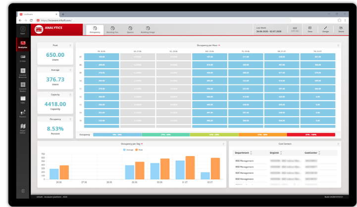
infsoft Analytics
