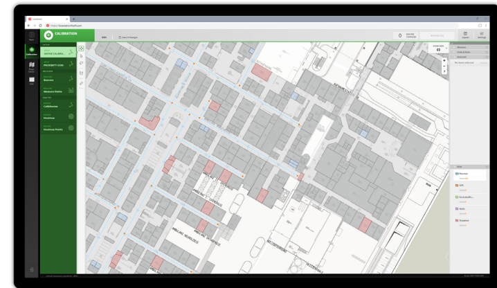
infsoft Calibration
